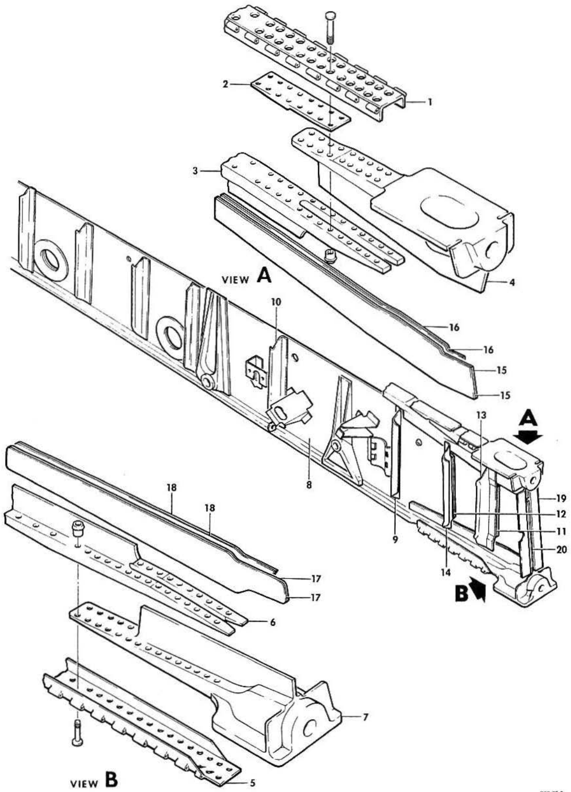
FIGURE 10-20. WING FRONT SPAR /SHEET 1 OF 2 SHEETS/
