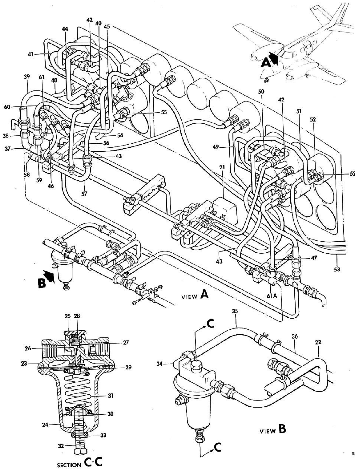
FIGURE 10-20. INSTRUMENT PANEL PLUMBING /SHEET 2 OF 3 SHEETS/
