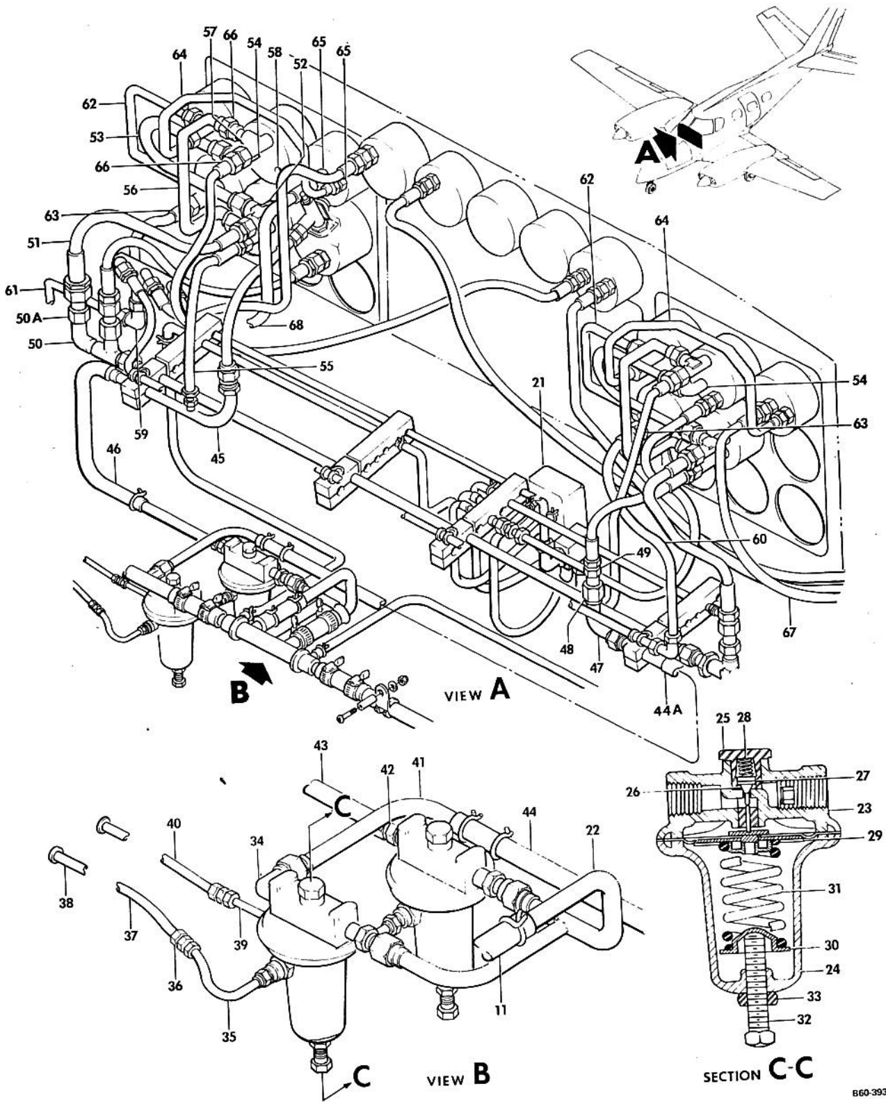
FIGURE 10-30. INSTRUMENT PANEL PLUMBING /SHEET 2 OF 3 SHEETS/
